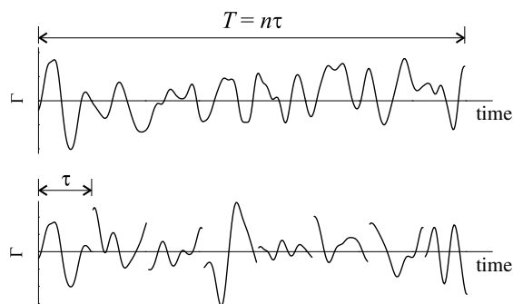
Fig. 2. Schematic representation of two molecular trajectories used in the test revealing correlations at time \tau ( \tau -test, see text). T represents the whole phase space of the molecular system. The top trajectory generates the 'original' signal, the bottom one generates the 'test' signal.
