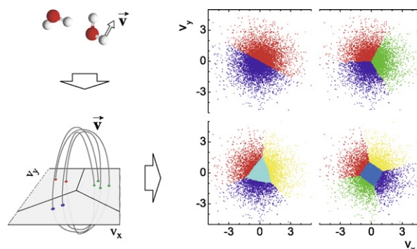
Fig. 5. The process of converting the continuous atomic velocity signal \mathbf{v} into symbolic sequence. On the right the symbolisation with 2, 3, 4, and 5 symbols are shown.
