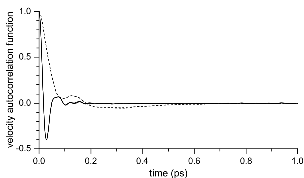
Fig. 1. Velocity autocorrelation function for oxygen (red) and hydrogen atoms of two water molecules calculated as time average over 2000 ps. The curves for the atoms of the same type are practically indistinguishable. (For interpretation of the references to colour in this figure legend, the reader is referred to the web version of this article.)
