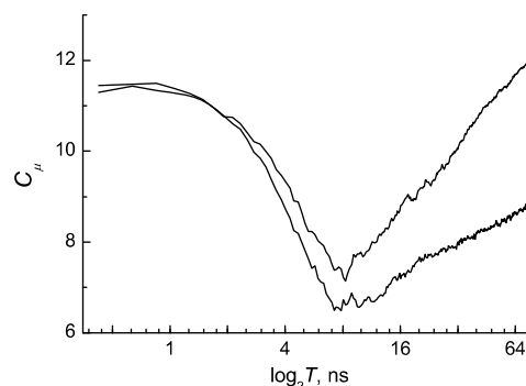
Fig. 3. Statistical complexity for the hydrogen velocity signal of bulk water. The original uninterrupted signal (red) and an ensemble consisting of 158 ps long parts are shown. (For interpretation of the references to colour in this figure legend, the reader is referred to the web version of this article.)
