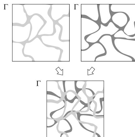
Fig. 4. Schematic representation of the molecular phase space \Gamma and 'network' formed by the trajectories for each uninterrupted part of the trajectory (see text). Upper two figures represent the networks for two individual parts while the lower figure demonstrates the larger phase space area of the combined network for the test signal phase space.
